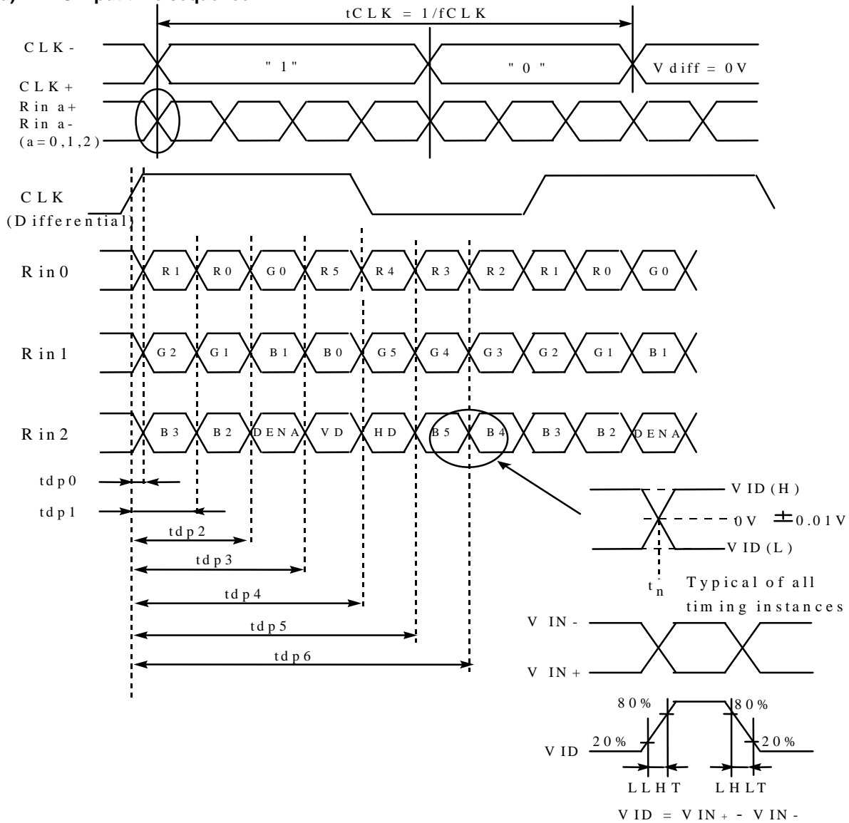
(a). LVDS input time sequence
