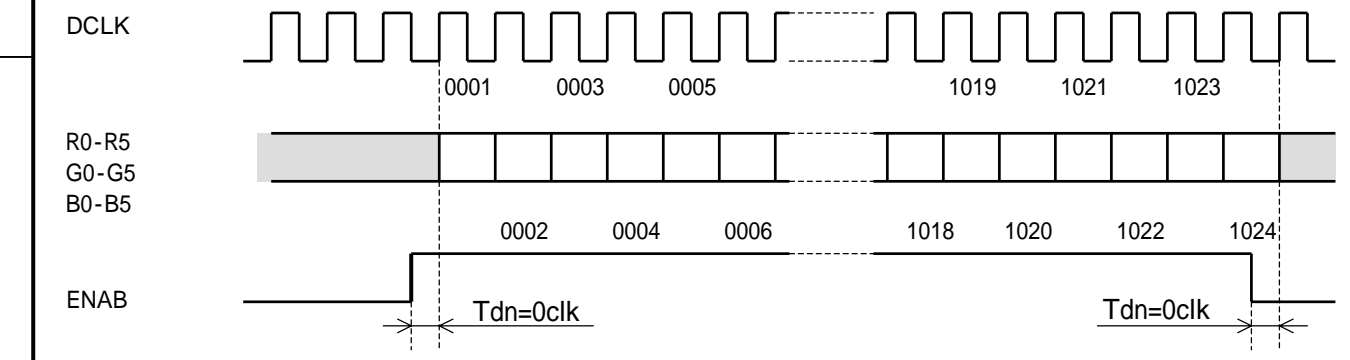
Figure 10-3 Input Signal Timing Chart
