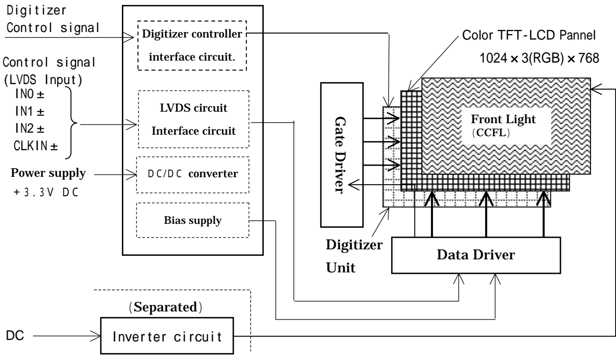
Figure 4-1 Block Diagram
