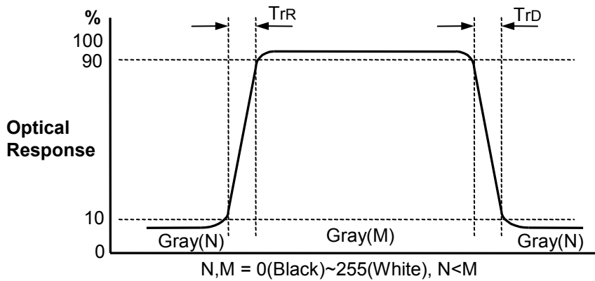
Figure 6. Response time
