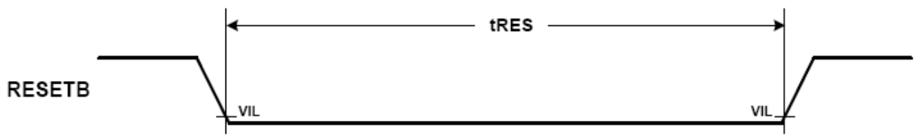
AC Characteristics(RESET timing)
