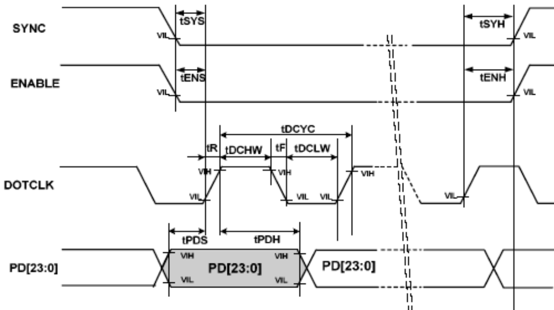
AC Characteristics
