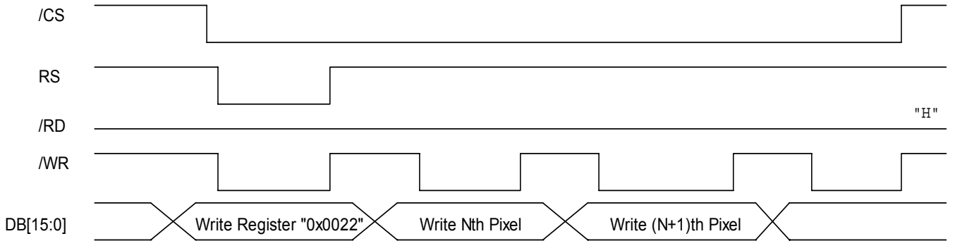
Figure 5.3.1 16-bit Write data for RGB 5-6-5-bits input(GRAM Write Timing)
